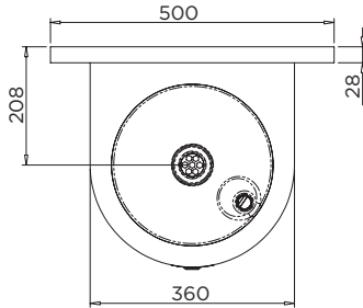
TW-BF-HF Fixed Spout Bottle Filler Hob Mounted
