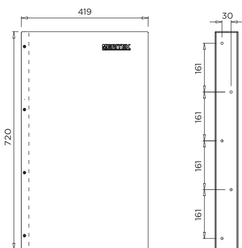
MODEL UPP Side and Rear Elevation
