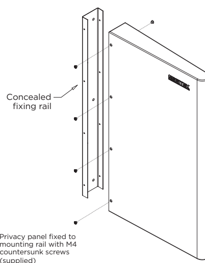
MODEL UPP Isometric View
