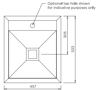
MODEL HBOBL-533 Plan
