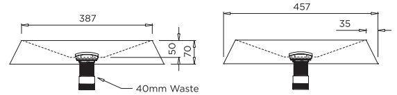
MODEL HBOBL-457 Front and Side Elevation
