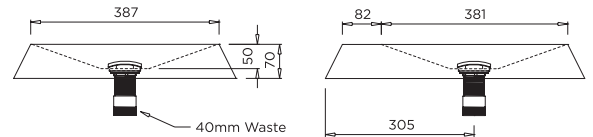
MODEL HBOBL-533 Front and Side Elevation
