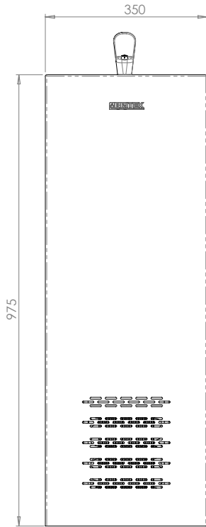
MODEL DSSR Front Elevation
