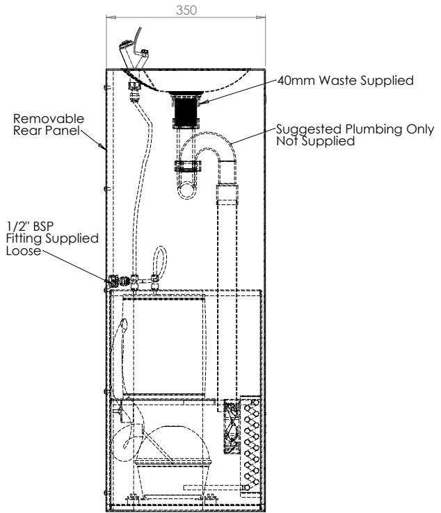
MODEL DSSR Side Elevation
