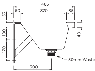
MODEL TABL Section
