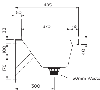
MODEL TABL-U Section
