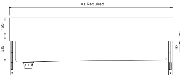
MODEL TABL Front Elevation and Plan
