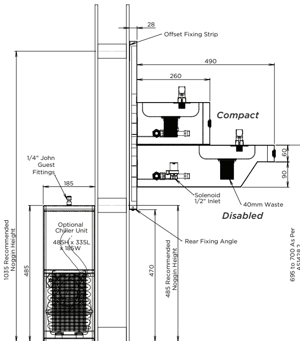
MODEL DDS2-R Side Elevation
