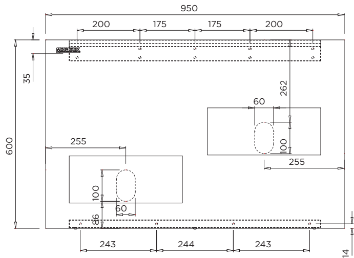
MODEL DDR2-R Plumbing Guide
