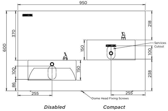
MODEL DDR2 Front Elevation
