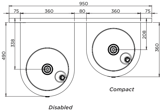
MODEL DDR2 Plan
