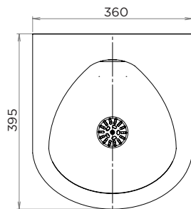
MODEL UR / URAM Plan
