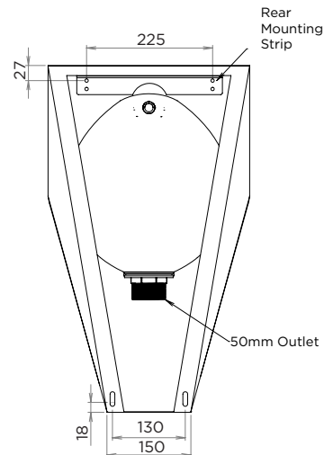
MODEL UR / URAM Rear Elevation
