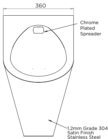
MODEL UR / URAM Front Elevation
