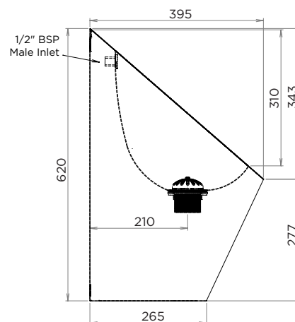
MODEL UR / URAM Section
