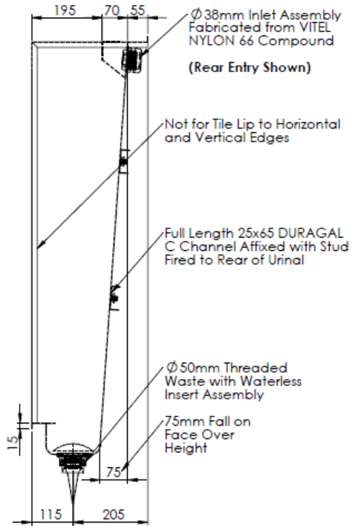
MODEL UESI-LF Typical Section
