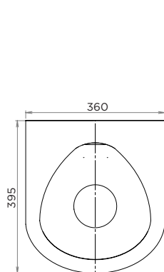
MODEL UBW Plan
