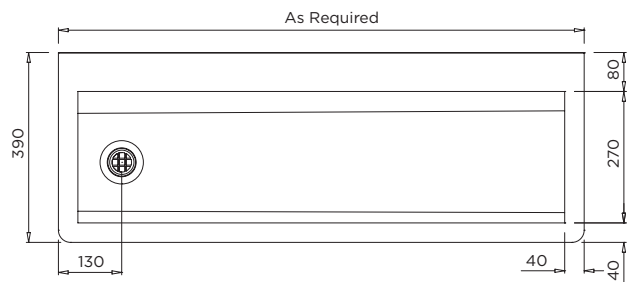
MODEL TWAL Plan
