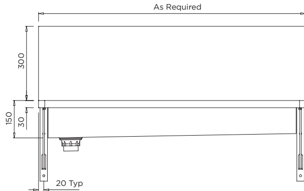
MODEL TWAL Front Elevation
