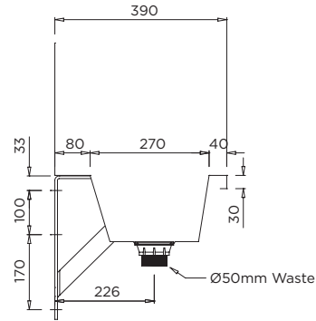
MODEL TWAL Side Elevation
