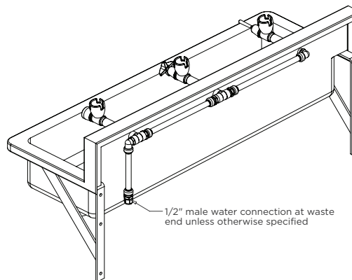
MODEL TPWDPD Rear Isometric View
