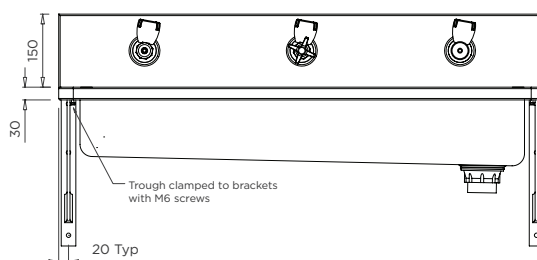
MODEL TPWDPD Section
