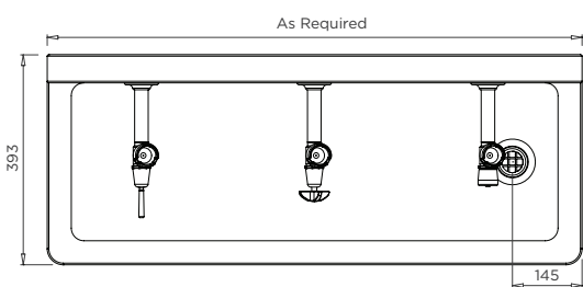
MODEL TPWDPD Plan
