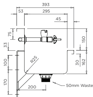
MODEL TPWDPD Section
