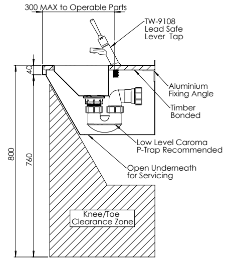
MODEL TPAHW-DDA Side Elevation
