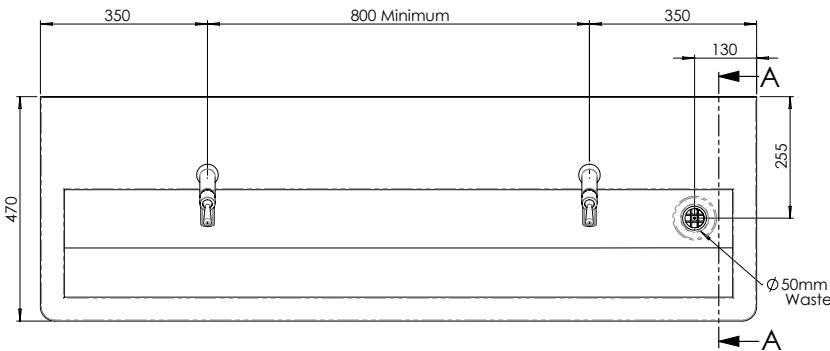
MODEL TPAHW-DDA Plan
