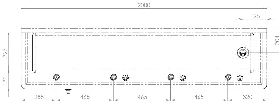
MODEL TP6 Plan
