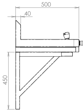
MODEL TP6 Side Elevation
