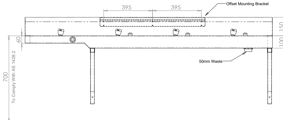
MODEL TP6 Front Elevation
