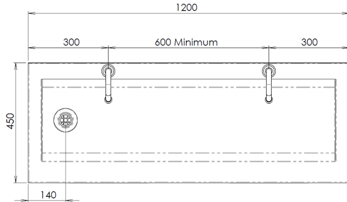
MODEL TMKO Plan
