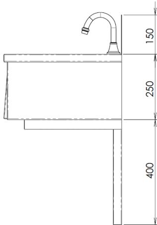
MODEL TMKO Side Elevation
