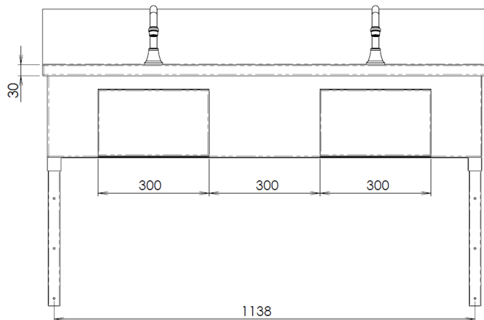
MODEL TMKO Front Elevation
