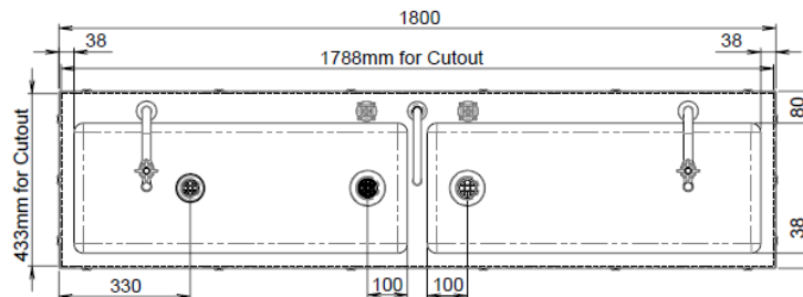
MODEL TCAI-PPC Plan and Front Elevation
