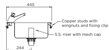
MODEL TCAI-PPC Side Elevation
