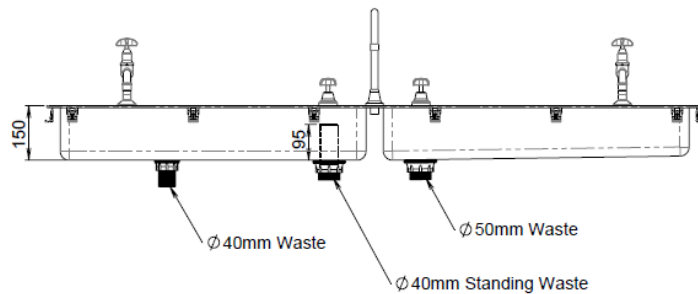
MODEL TCAI-PPCH Plan and Front Elevation
