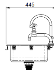
MODEL TCAI-PPCH Side Elevation
