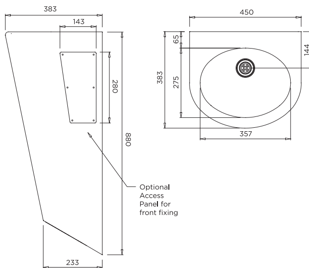
MODEL SPBO Side Elevation and Plan
