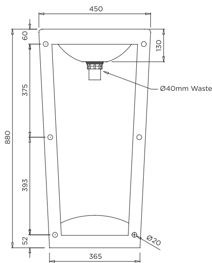
MODEL SPBO Rear Elevation
