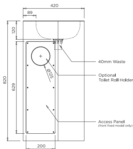
MODEL SPB Side Elevation
