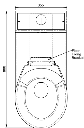
MODEL PTSDC Plan
