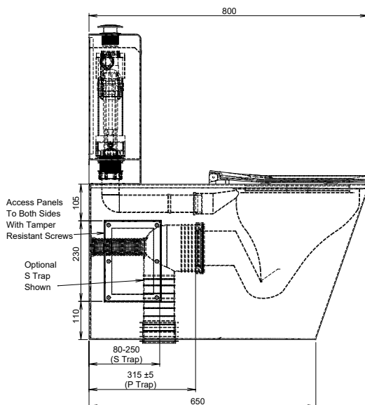
MODEL PTSDC Side and Rear Elevation
