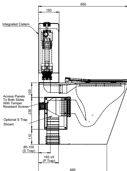
MODEL PTSAM Side and Rear Elevation
