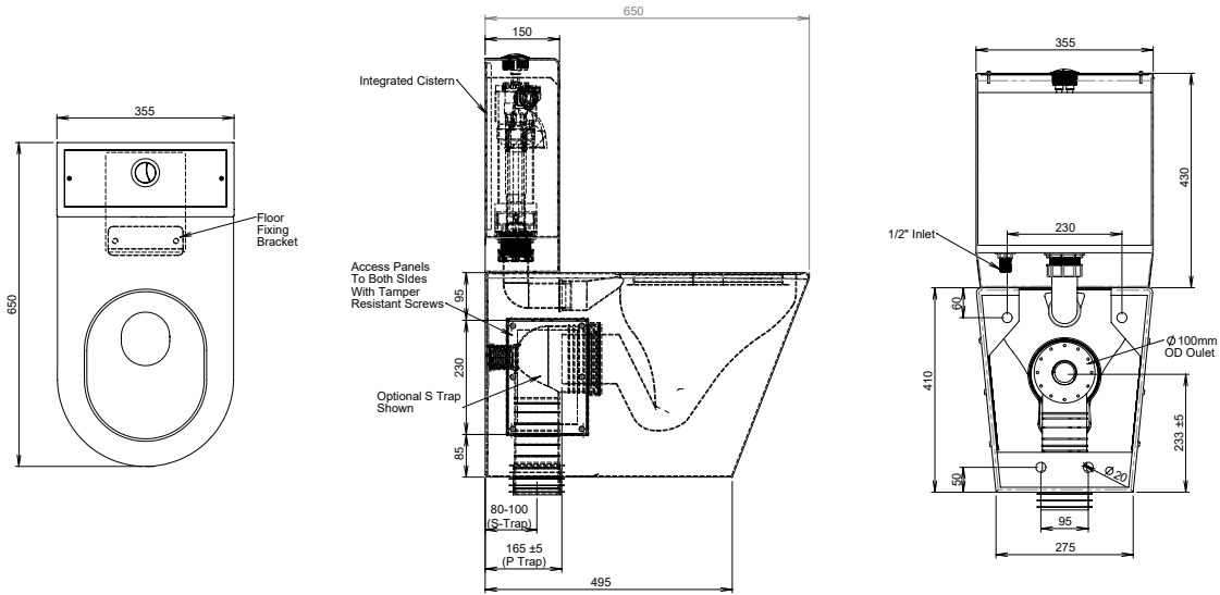
MODEL PTSC Plan, Side Elevation, Rear Elevation
