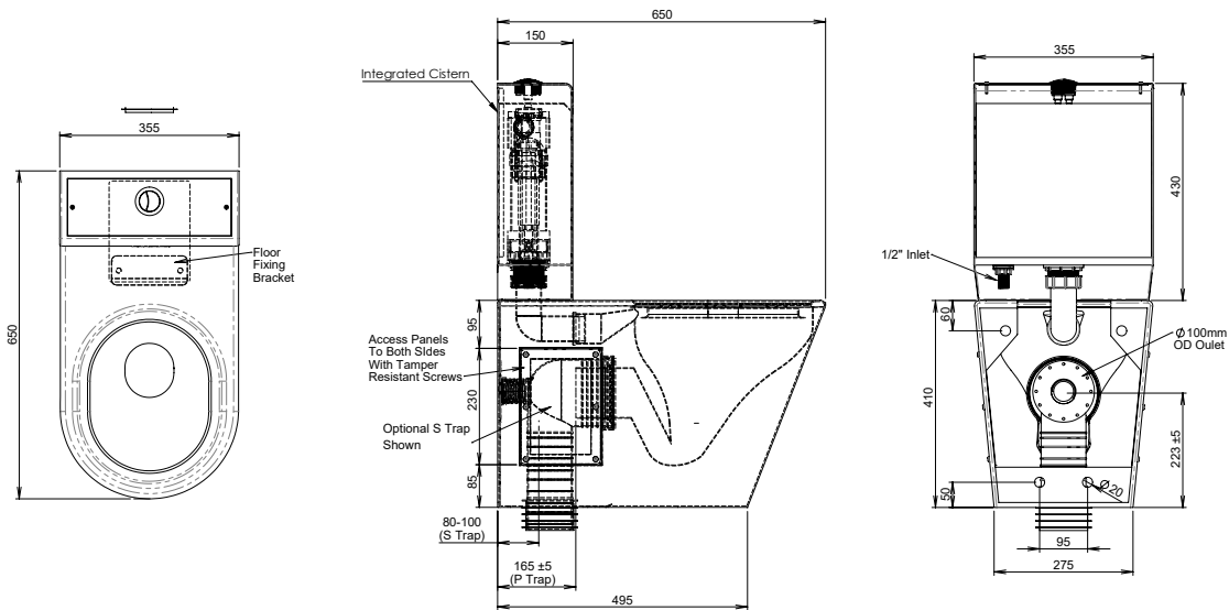
MODEL PTSG Plan, Side Elevation, Rear Elevation
