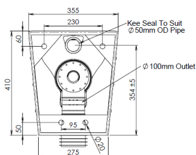
MODEL PGS Side and Rear Elevation
