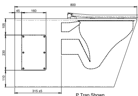
P Trap Shown
