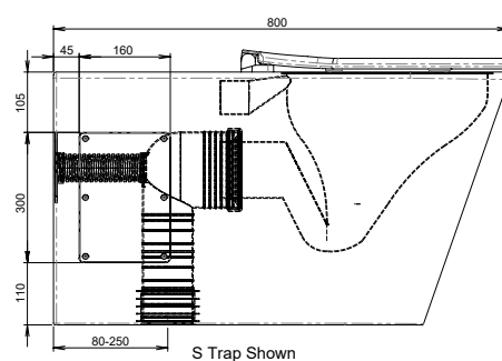
S Trap Shown
