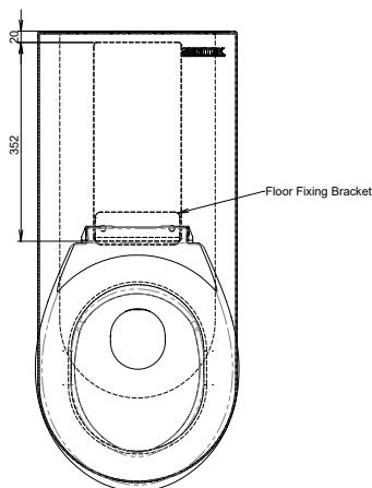
MODEL PCDS / PCDP Plan
