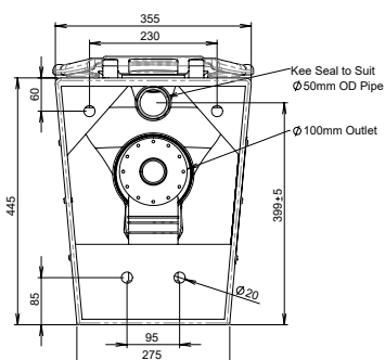
MODEL PCDS Side and Rear Elevation
