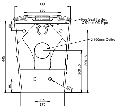
MODEL PCDP Side and Rear Elevation
