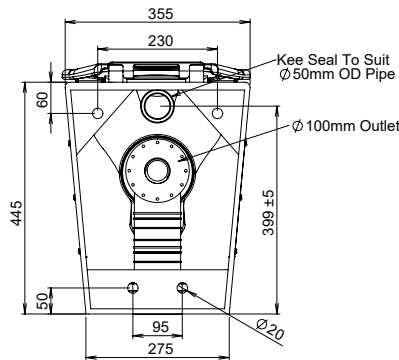
MODEL PCAMS Side and Rear Elevation
