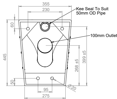
MODEL PCAMP Side and Rear Elevation
