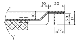
A Detail
