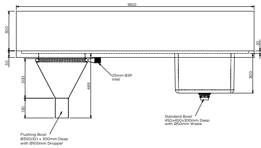
MODEL LDUS-A Front Elevation
