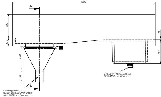
MODEL LDUS-B Front Elevation
