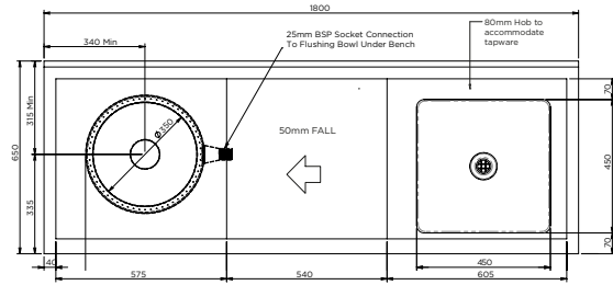
MODEL LDUS-B Plan
