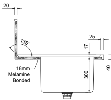
MODEL LAB-WS Side Elevation
