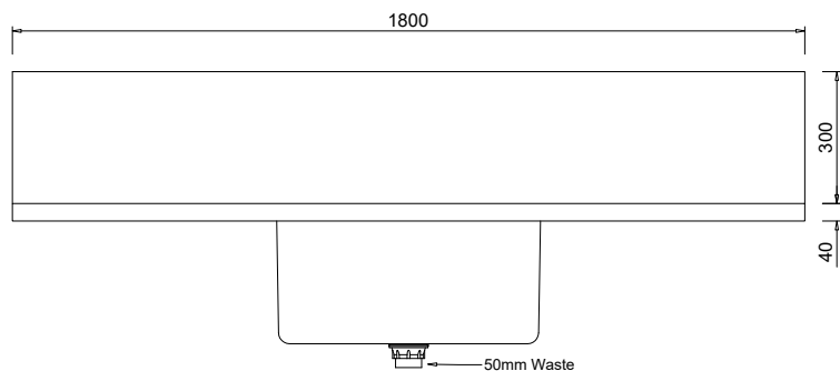
MODEL LAB-WS Front Elevation
