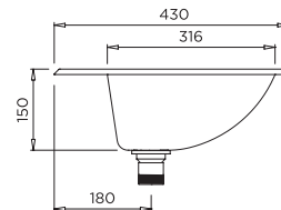
MODEL HBRE Side Elevation
