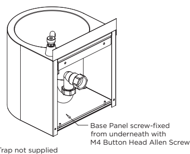
MODEL HBVR Isometric View (Rear)
