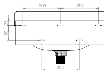
MODEL HBS Rear Elevation
