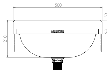
MODEL HBS Front Elevation
