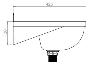
MODEL HBS Side Elevation
