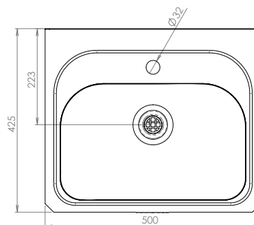
MODEL HBS Plan
