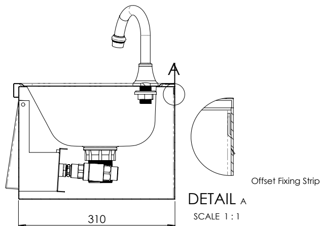
MODEL HBKOC Section
