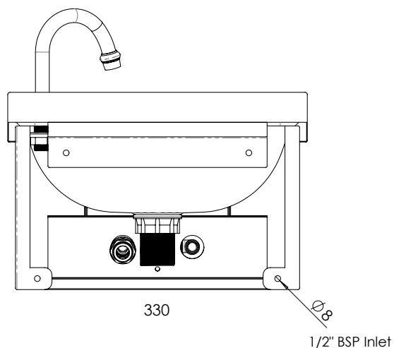
MODEL HBKOC Rear Elevation
