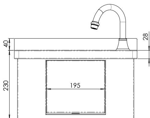
MODEL HBKOC Front Elevation
