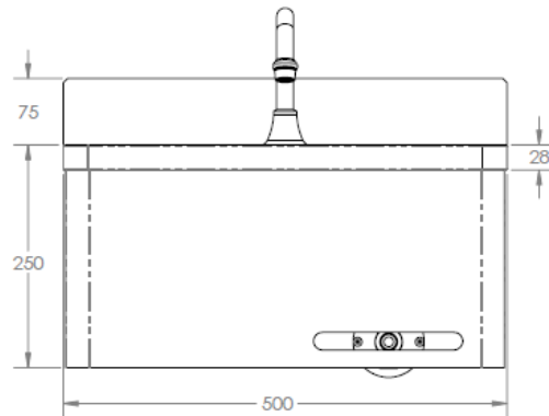
MODEL HBFWS Front Elevation
