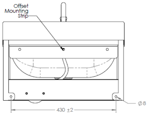
MODEL HBFWS Rear Elevation
