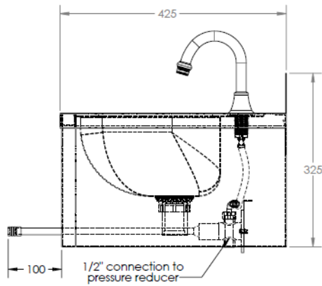
MODEL HBFWS Side Elevation
