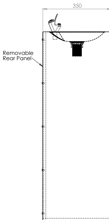
MODEL DSS Side Elevation
