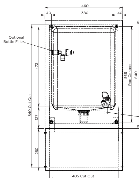
MODEL DRDC-FF Side Elevation, Front Elevation and Plan
