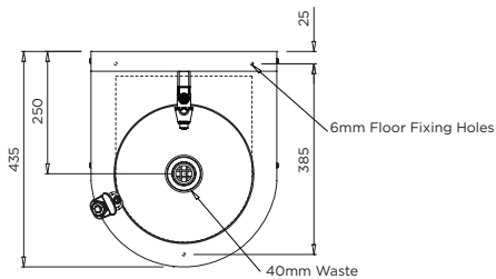
MODEL DFRE Plan
