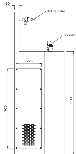
MODEL DFRE Side Elevation
