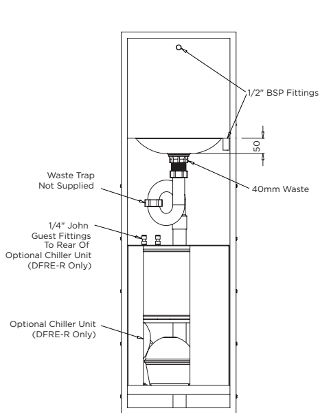
MODEL DFRE Rear Elevation and Front Elevation
