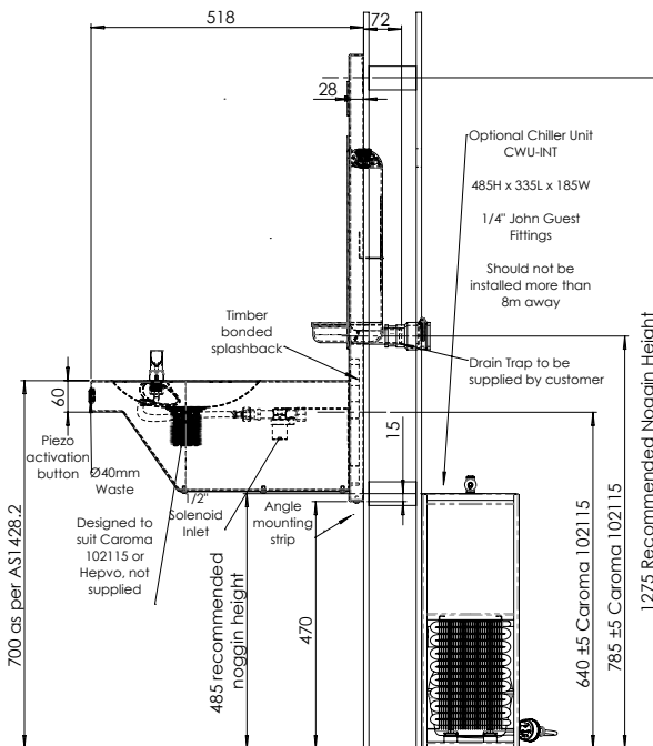
MODEL DDR1-D-HFBF Side
