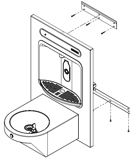
MODEL DDR1-D-HFBF Joggle Strip
