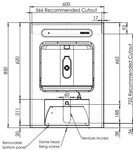
MODEL DDR1-D-HFBF Front Elevation
