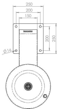
MODEL DDIS Plan, Front Elevation
