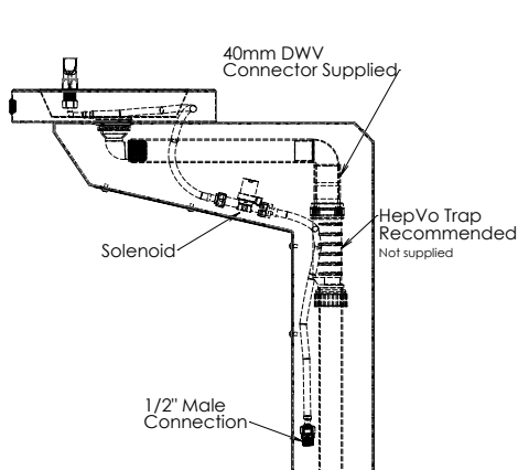
MODEL DDIS Side Elevation
