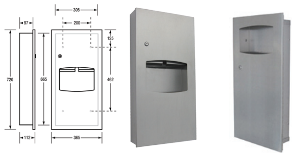
Paper Towel Dispenser & Waste Receptacle Model
