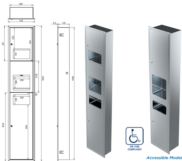
Accessible Model BTX-03-23
