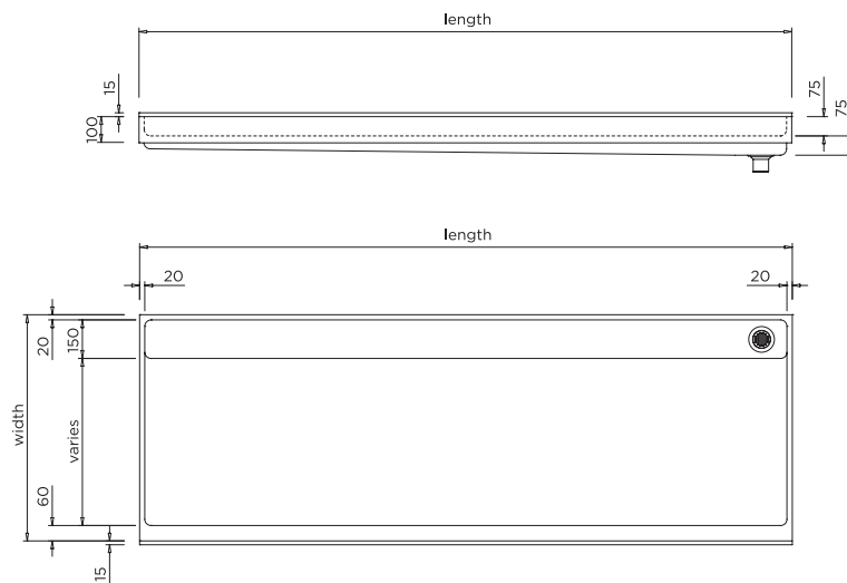
MODEL BSBM-C Plan and Front Elevation
