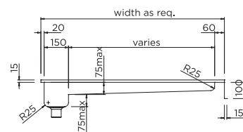
MODEL BSBM-C Side Elevation
