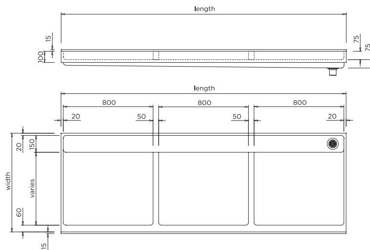
MODEL BSBM-MC Plan and Front Elevation
