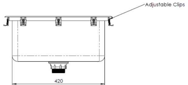
MODEL BB1 Front Elevation
