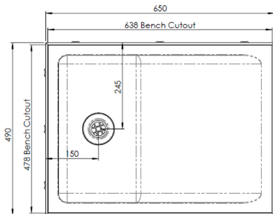
MODEL BB1 Plan
