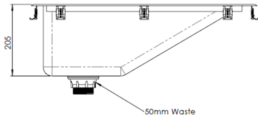
MODEL BB1 Side Elevation
