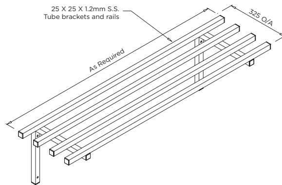
MODEL SHELF-T Isometric View
