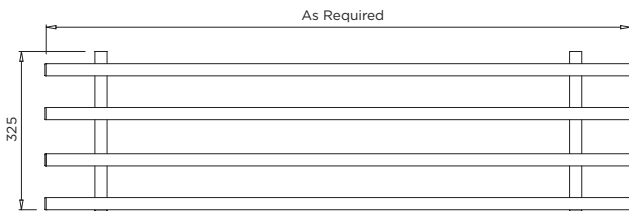
MODEL SHELF-T Front Elevation
