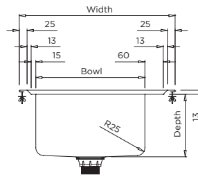
MODEL LSSEB Section
