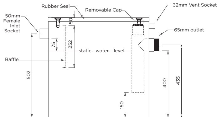
MODEL OSGI Side Elevation
