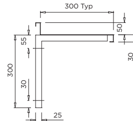
MODEL SHELF-S Sealed Upstand Section
