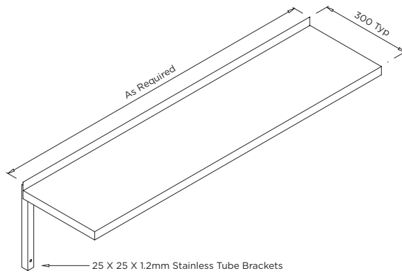
MODEL SHELF-S Isometric View
