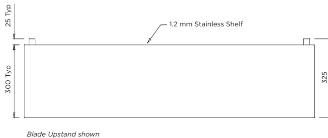
MODEL SHELF-S Plan
