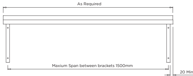
MODEL SHELF-S Front Elevation and Side Elevation
