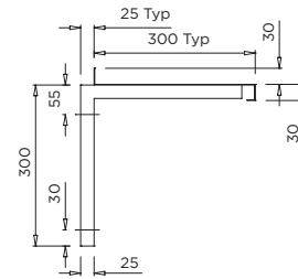
MODEL SHELF-S Blade Upstand Section
