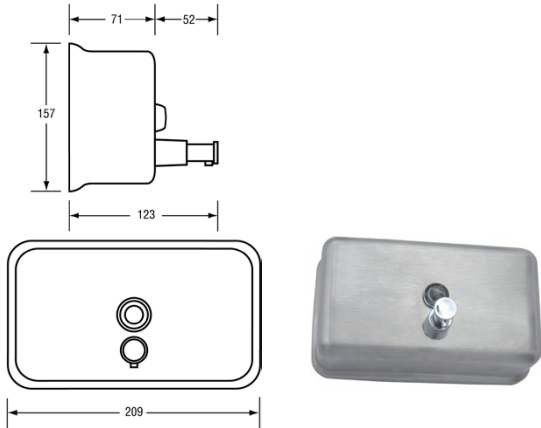
BTX-05-019 Horizontal Liquid Soap Dispenser S.S.
