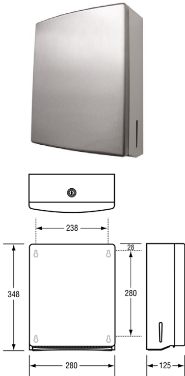
BTX-04-014 S.S. Contour Paper Towel Dispenser
